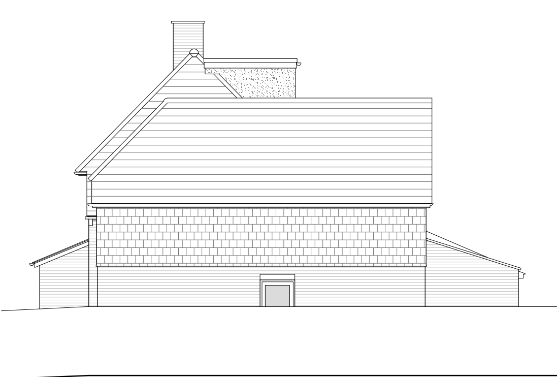
East Elevation
